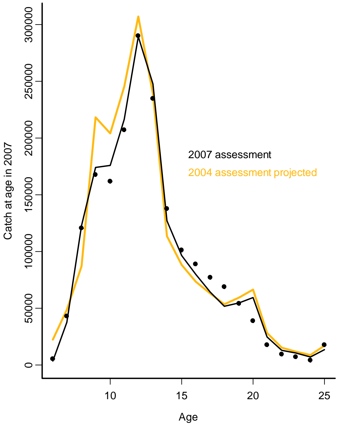
Fig 6a. Observed commercial catch at age of females in 2007 (points) and predicted catch at age from the 2007 assessment and from a blind projection of the 2004 assessment.
