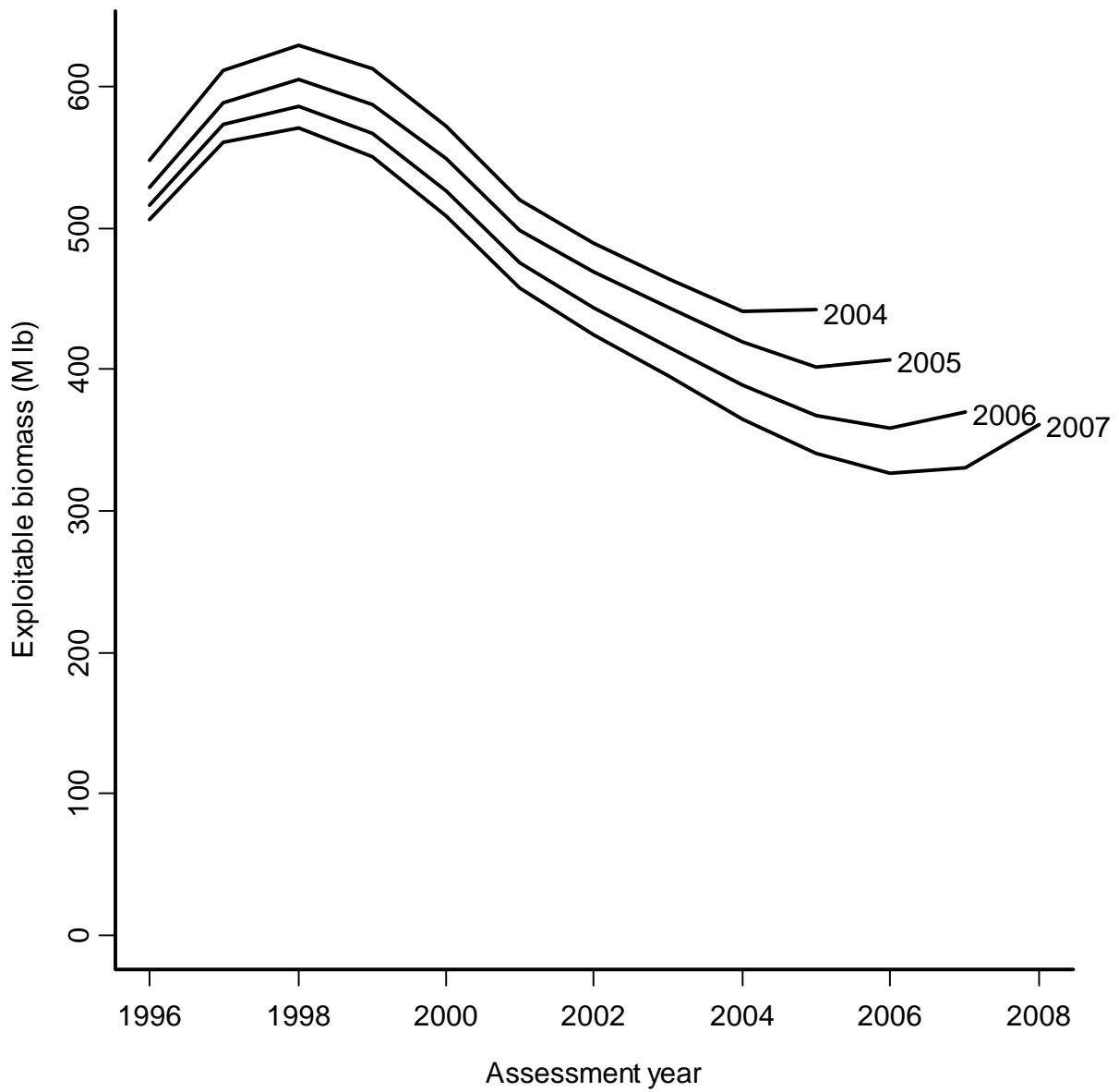
Fig. 5. Retrospective performance of the assessment. Each line is the biomass trajectory estimated by the model fitted to data from 1996 through the labeled last year.
