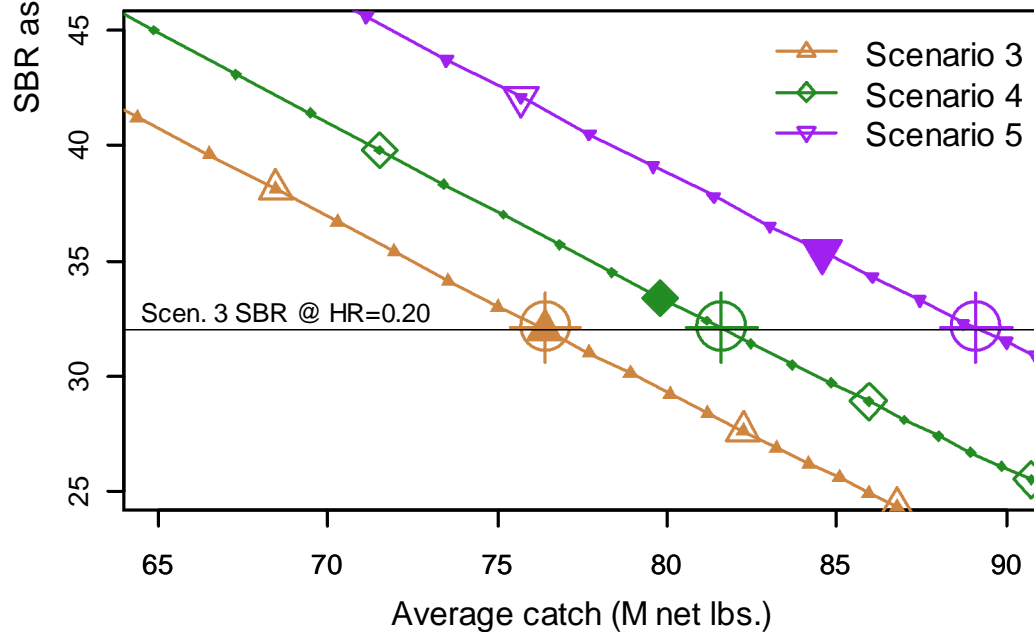
Figure 4. Results of Spawning Biomass per Recruit (SBR) analysis. See text for definition of Scenarios. Panel a shows the Average Catch vs. SBR curves as a function of increasing harvest rate. The upper left point of each curve is a harvest rate of 0.0; each dot down the curve represents an increase of 0.01; the large dots are in multiples of 0.05 and the large shaded dot indicates a harvest rate of 0.20. The horizontal line is the SBR for Scenario 3 at harvest rate of 0.20. Panel b contains the same data as Panel a but is zoomed into the region of interest without the first two Scenarios plotted. The bullseyes show the harvest rate that reduces SBR to the same level as a harvest rate of 0.20 in Scenario 3.
