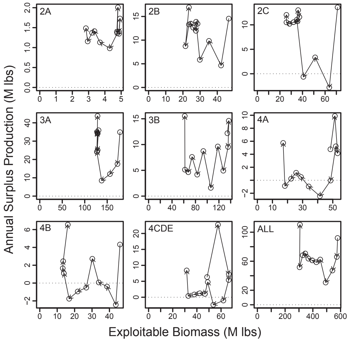
Figure 2. Relationship between Exploitable Biomass and Annual Surplus Production over the period 1997 (originating circle) to 2008 (concluding circle).
